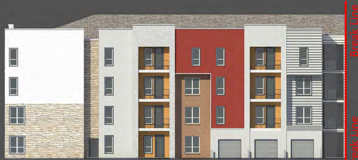
9% Face Brick, 61% Thin Brick, 4% Cultured Stone, 26% Wood Siding 28% Windows SF facing Public Right of Way Building Number 5 Building Type IV 4% Wood Accent Trim Break Line Break Line (09) South Elevation
