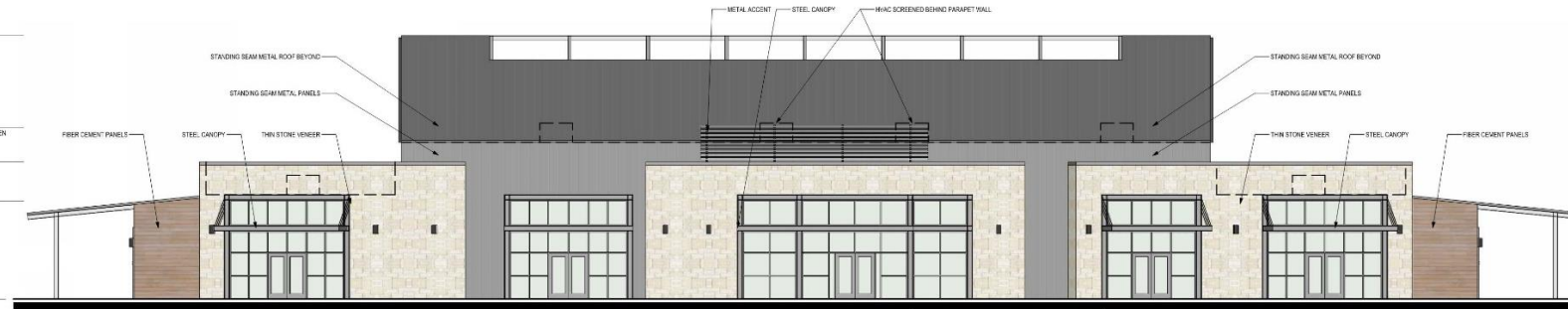
01 EAST ELEVATION 1/8" = 1'-0"
