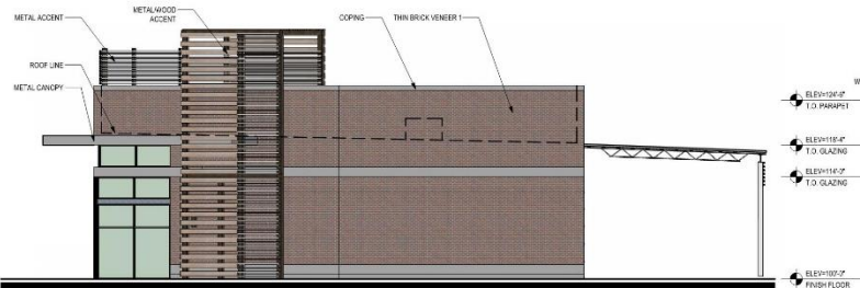
04 SOUTH ELEVATION 1/8" = 1'-0"
