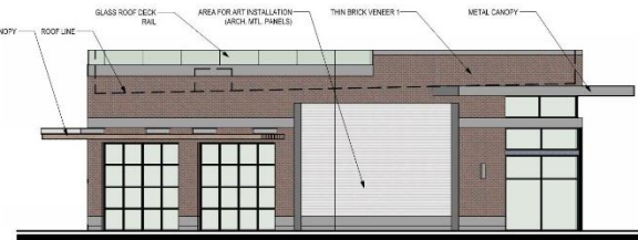
03 NORTH ELEVATION 1/8" = 1'-0"
