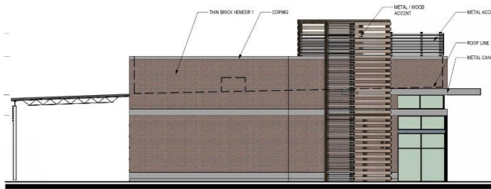
04 SOUTH ELEVATION 1/8" = 1'-0"
