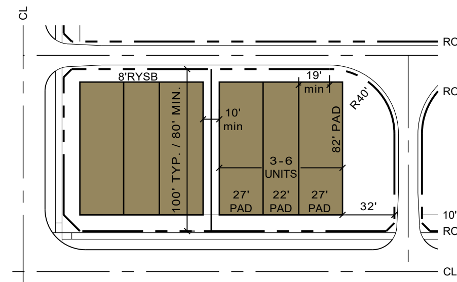
STANDARD TOWNHOME LOT
