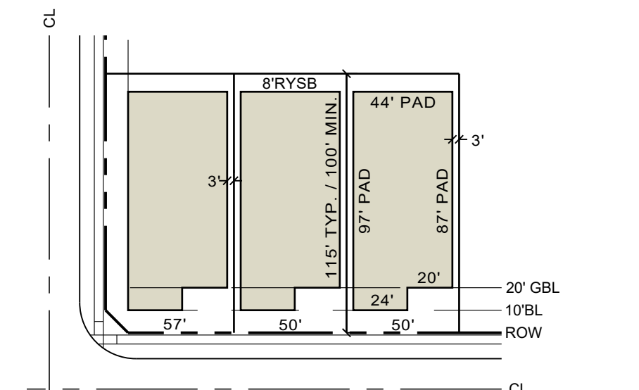
STANDARD 50' LOT (FRONT ENTRY)
