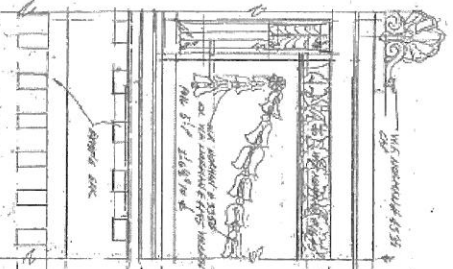
3 TYPICAL CORNICE 1/8" = 1'-0"
