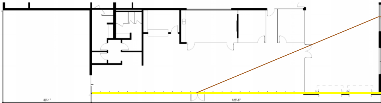
2a A4 Partial Floor Plan - South 3/32" = 1'-0"
