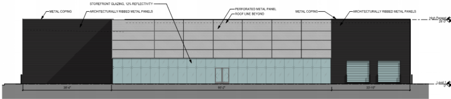
2 A4 South Elevation - Color 3/32" = 1'-0"
