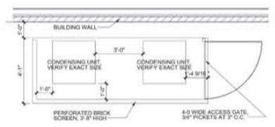
05 HVAC Condensing Unit Screening Plan 1/2"=1'-0"
