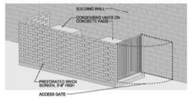
06 HVAC Condensing Unit Screening Isometric View not to scale
