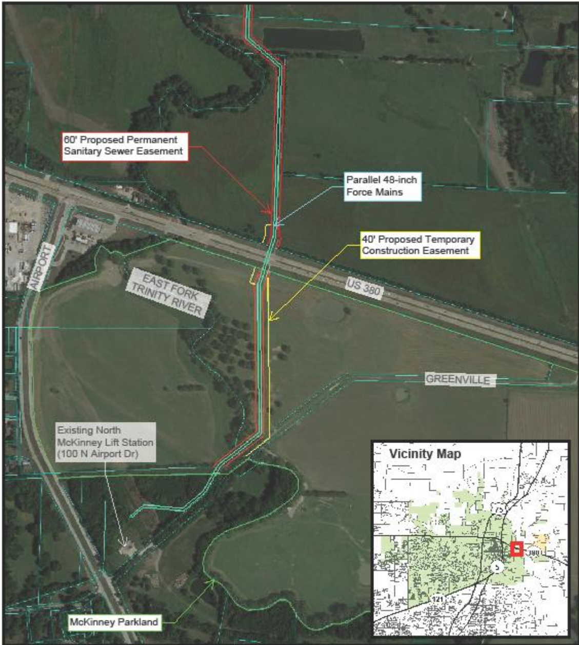
Exhibit A: North McKinney Transfer Force Main McKinney Parkland Alignment
