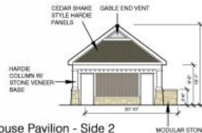
Poolhouse Pavilion - Side 2 Total Masonry: 73% Stone: 52% Brick: 21% Shake: 23% Trim: 4%
