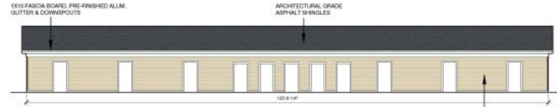
Storage Rear Masonry (Brick): 2% Lap: 94% Trim 4%
