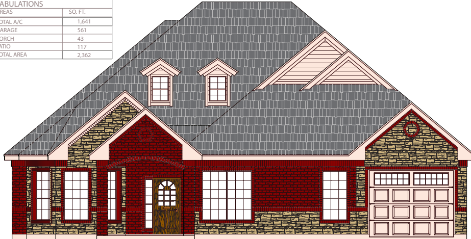
1 FRONT ELEVATION SCALE: NTS
