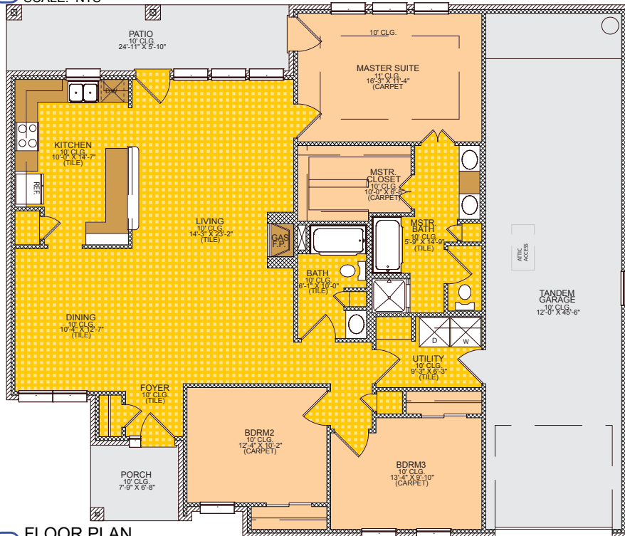
2 FLOOR PLAN SCALE: NTS
