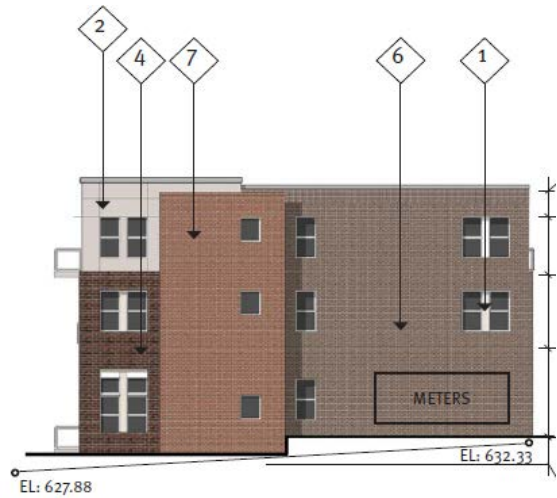
02 BLOCK B WEST ELEVATION (TENNESSEE ST)
