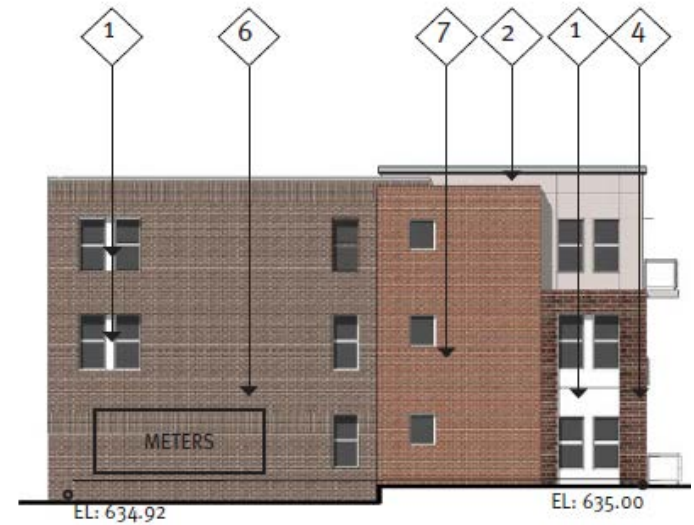
02 BLOCK B SOUTH ELEVATION (ANTHONY ST)
