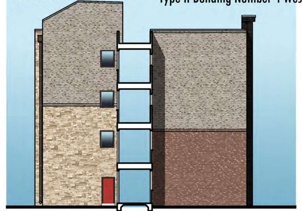
WEST ELEVATION
