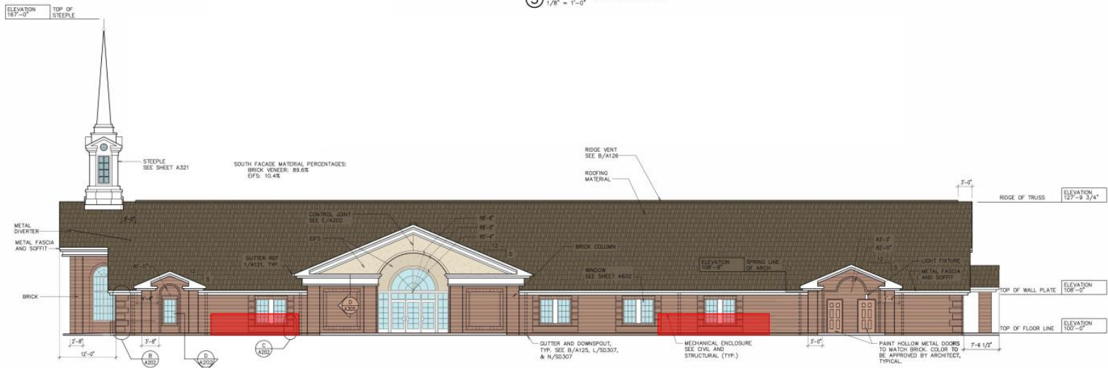
1 SOUTH ELEVATION 1/8" = 1'-0"
