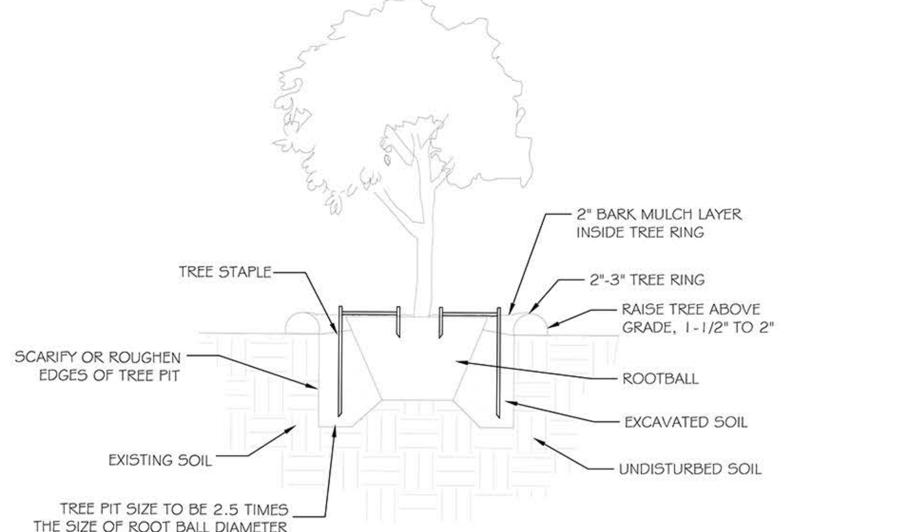
1 TREE PLANTING DETAIL 1" = 1'-0"
