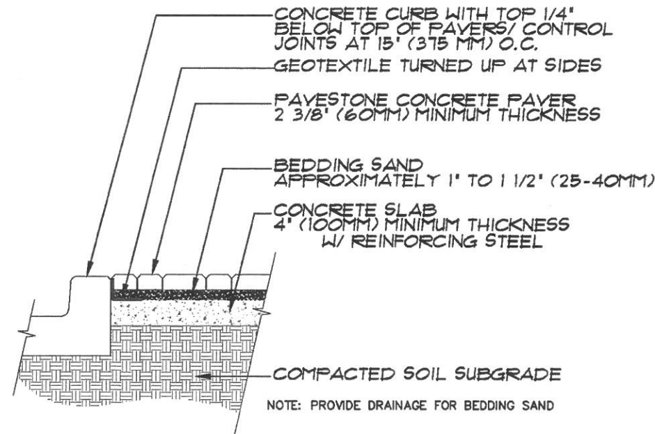
(C) SIDEWALK PAVER ON CONCRETE BASE NOT TO SCALE
