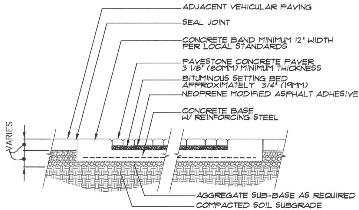
(A) CROSSWALK ON CONCRETE BASE NOT TO SCALE
