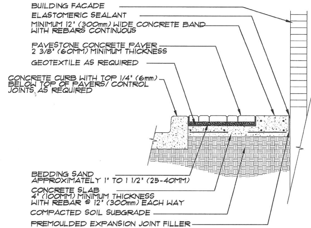
(B) CONCRETE BORDER ADJACENT TO BUILDING FACADE NOT TO SCALE
