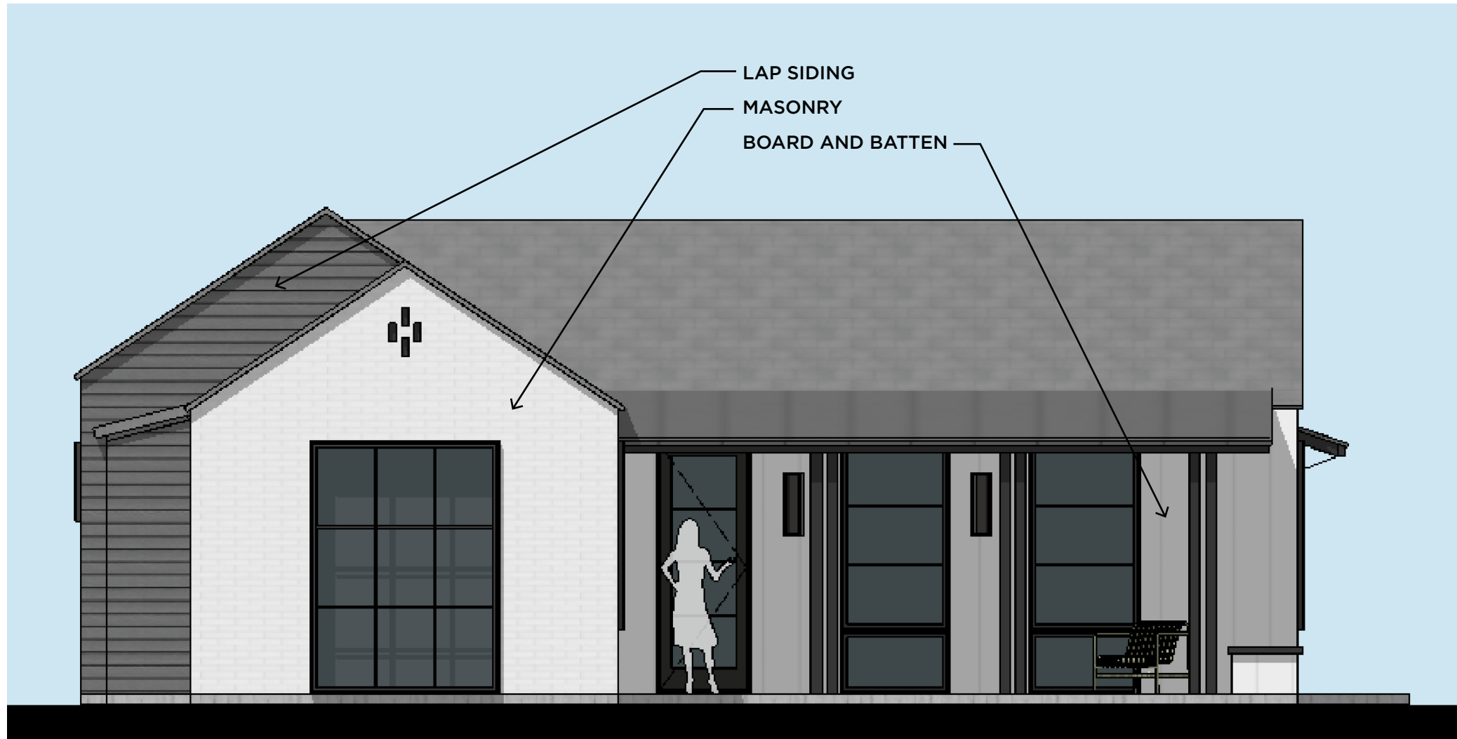
ELEVATION - FRONT
