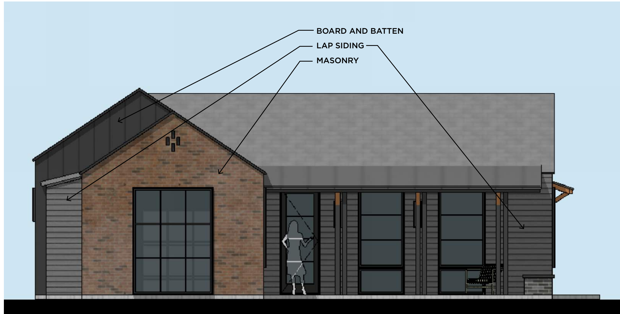
ELEVATION - FRONT
