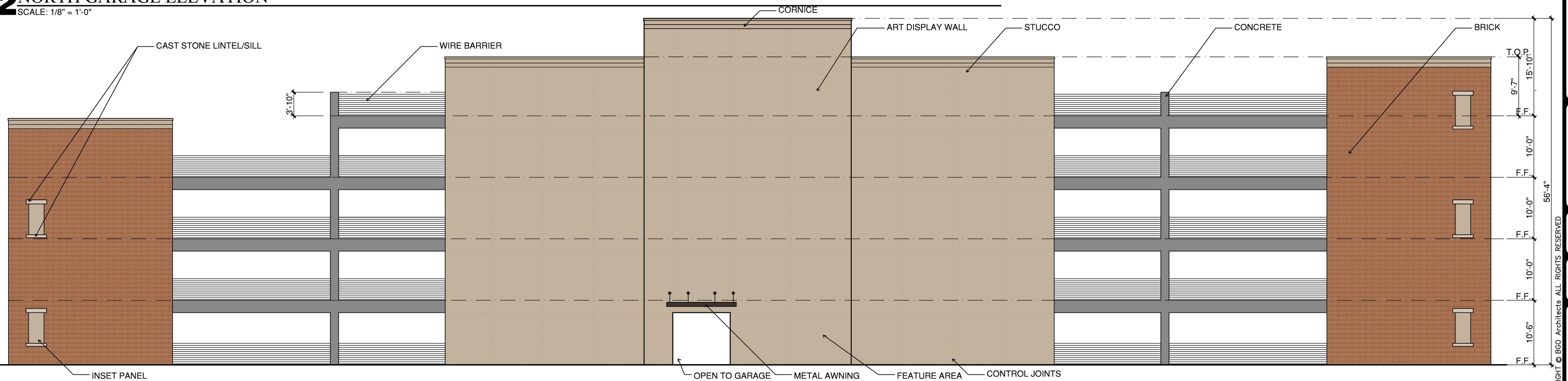
1 SOUTH GARAGE ELEVATION SCALE: 1/8" = 1'-0"
