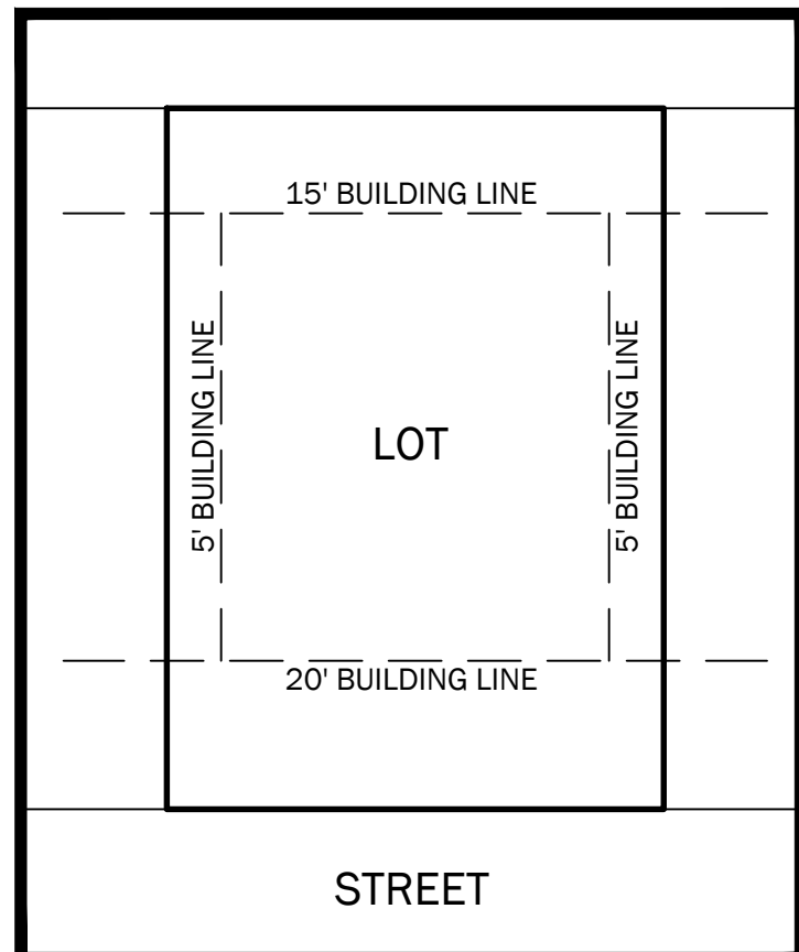
LOT SETBACK DETAIL NOT TO SCALE
