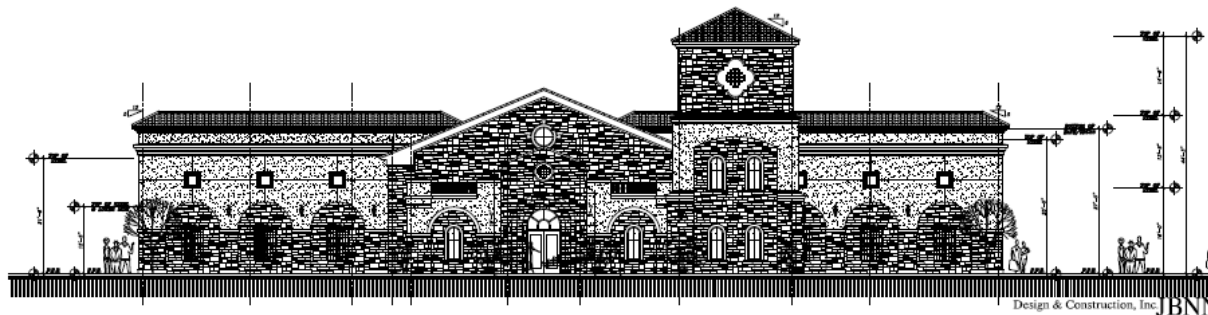
FRONT ELEVATION
