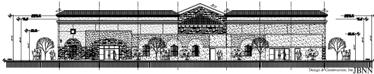
REAR ELEVATION
