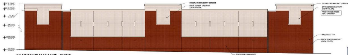
01 EXTERIOR ELEVATION - SOUTH Scale: 3/8"=1'-0"
