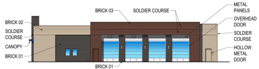
SIDE ELEVATION
