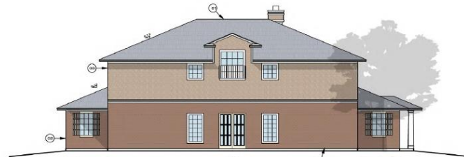
CLUBHOUSE REAR ELEVATION
