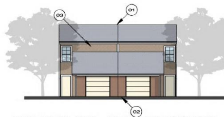
BUILDING #12 - SOUTH ELEVATION
