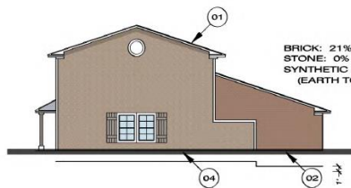
BUILDING #12 - WEST ELEVATION - EAST SIMILAR
