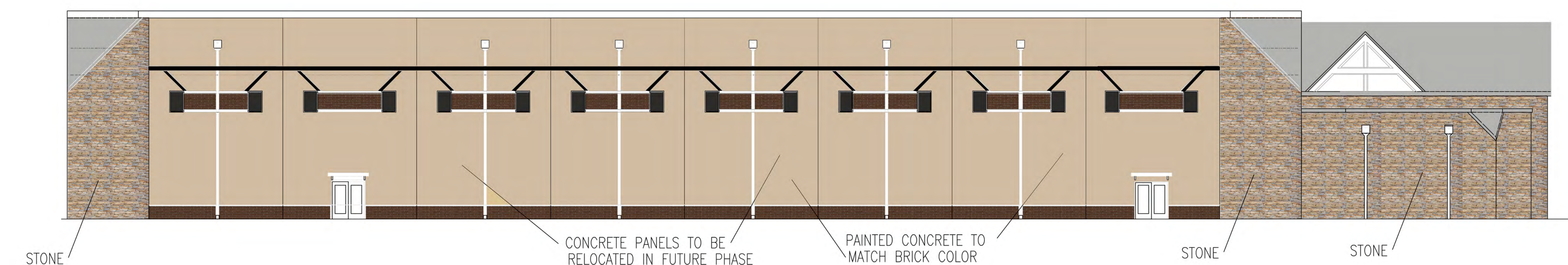
SOUTH ELEVATION
