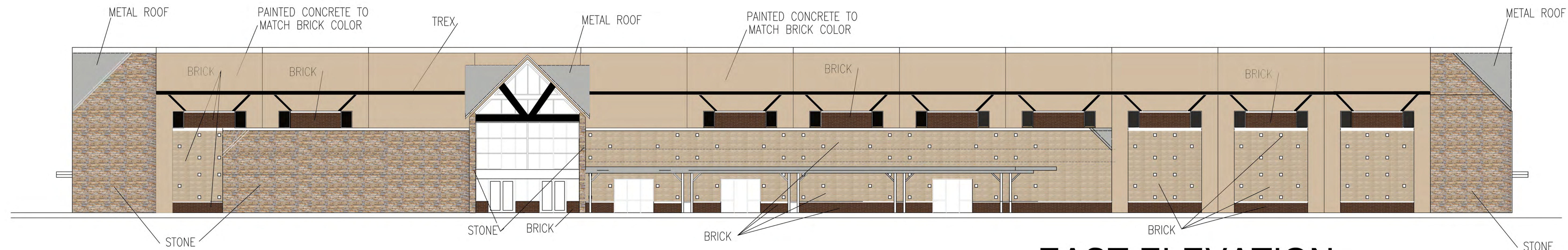
EAST ELEVATION
