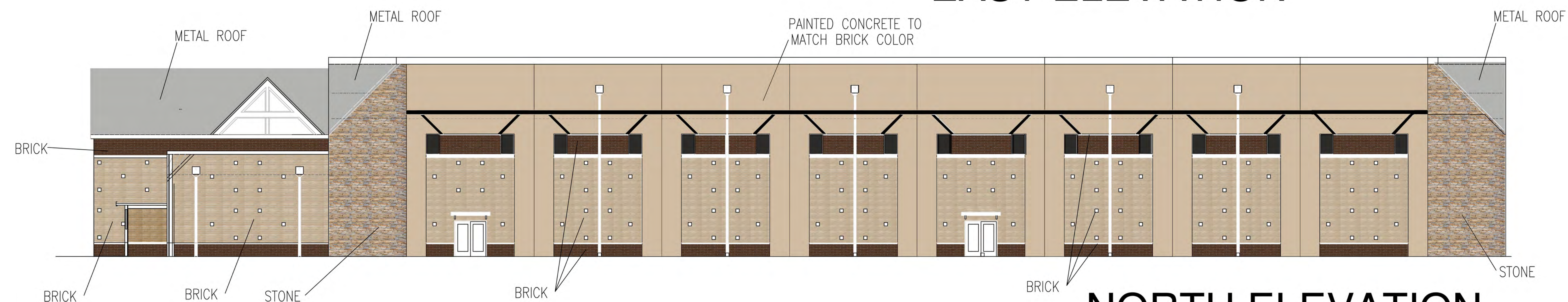
NORTH ELEVATION
