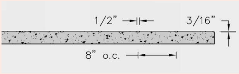
VERTICAL WOOD BOARD CONCRETE FORMLINER PATTERN
