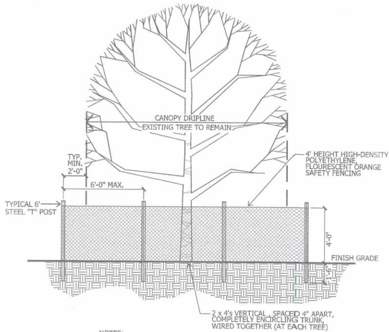
DETAIL L1.01 EXISTING TREE PROTECTION DETAIL not to scale
