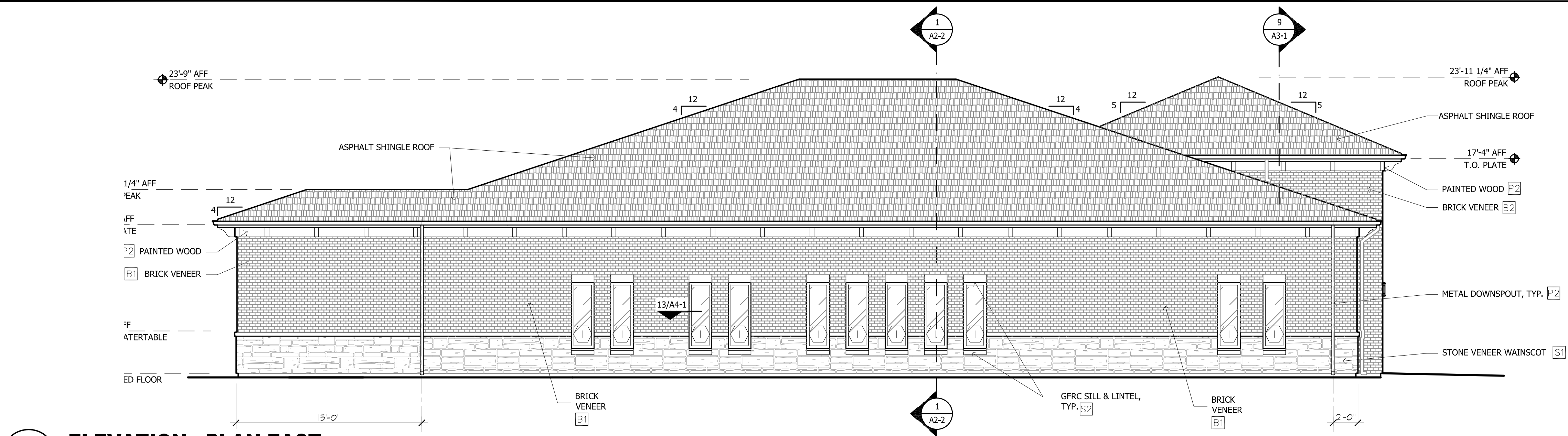
1 ELEVATION - PLAN EAST SCALE: 3/16" = 1'-0"
