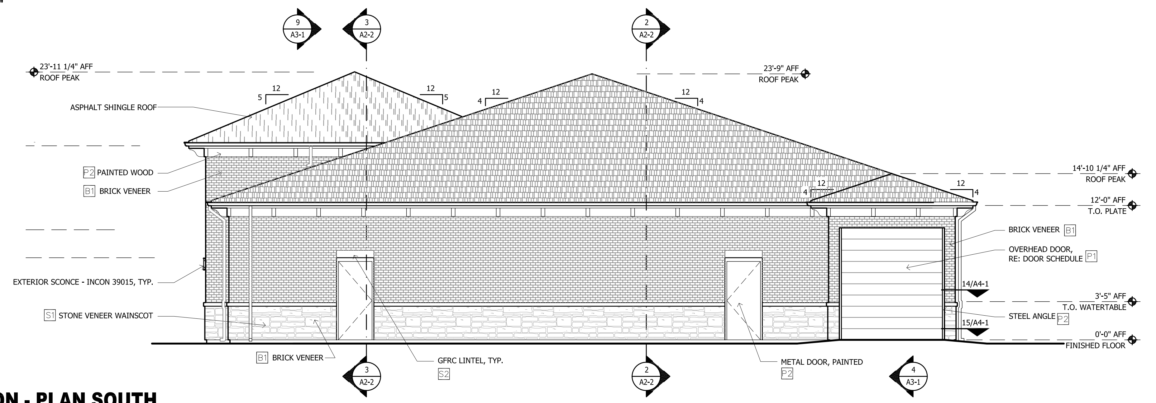
4 ELEVATION - PLAN SOUTH SCALE: 3/16" = 1'-0"
