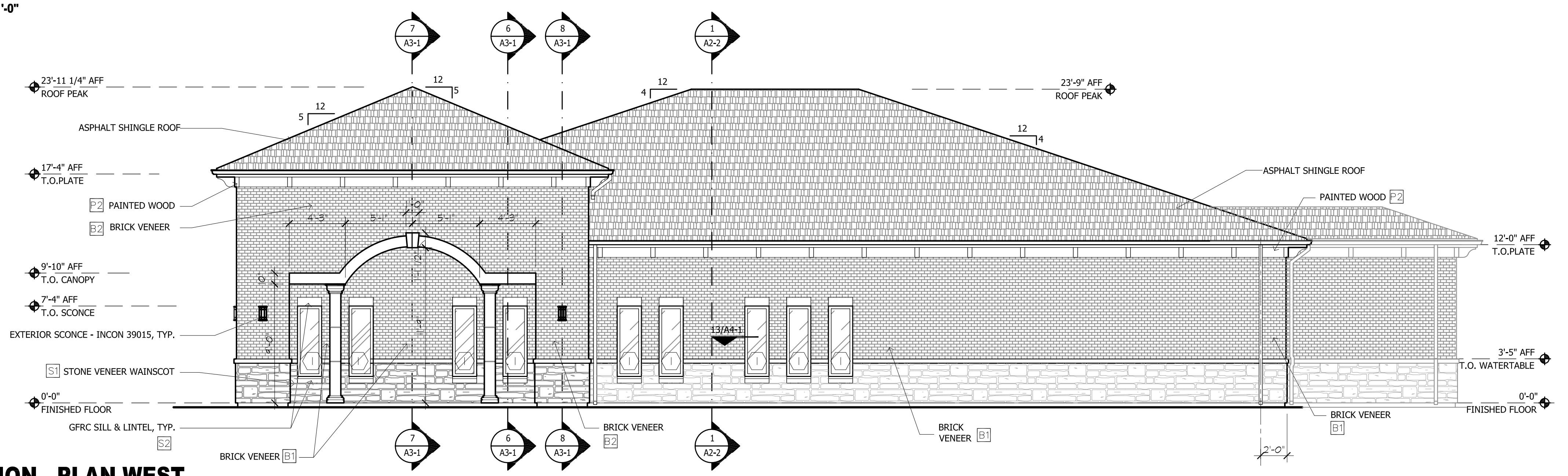
3 ELEVATION - PLAN WEST SCALE: 3/16" = 1'-0"
