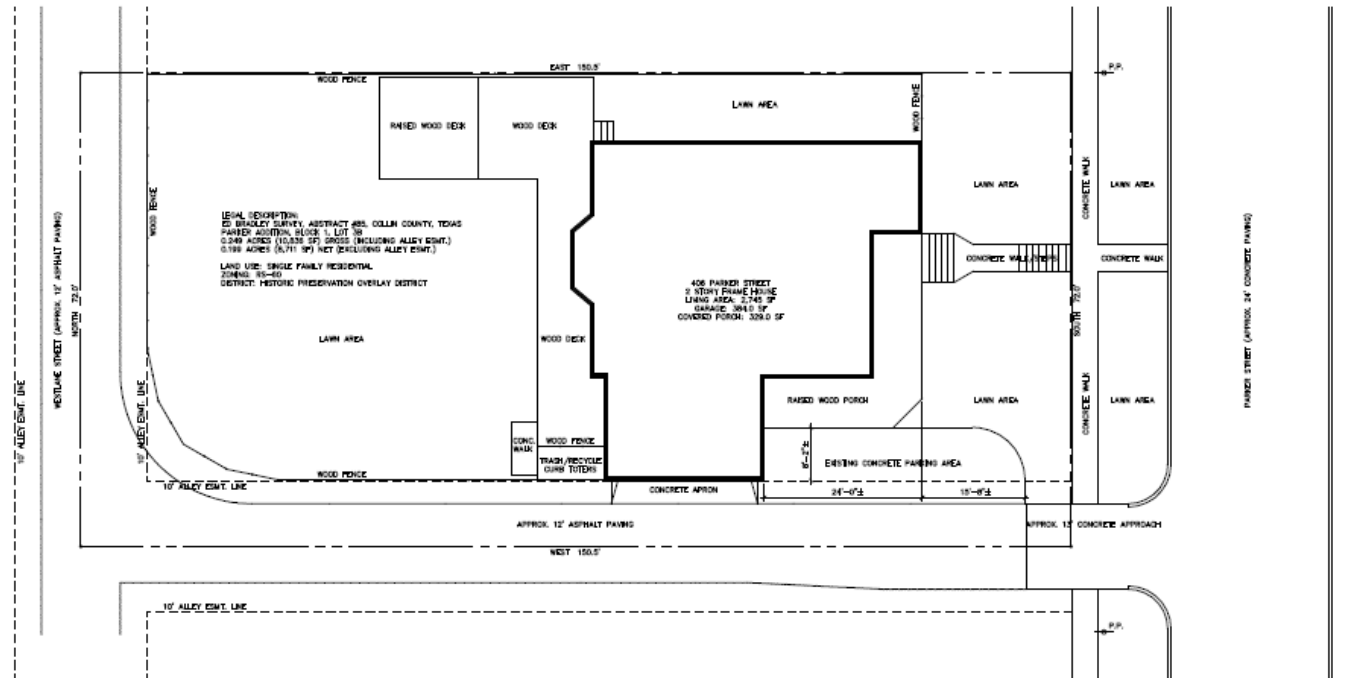
1 EXISTING SITE PLAN 1/8" = 1'-0"
