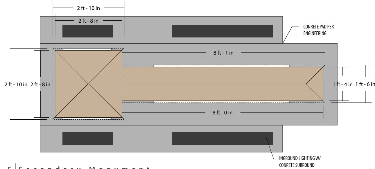
F | Secondary Monument .02 | Scale: 1/2" = 1' - 0"
