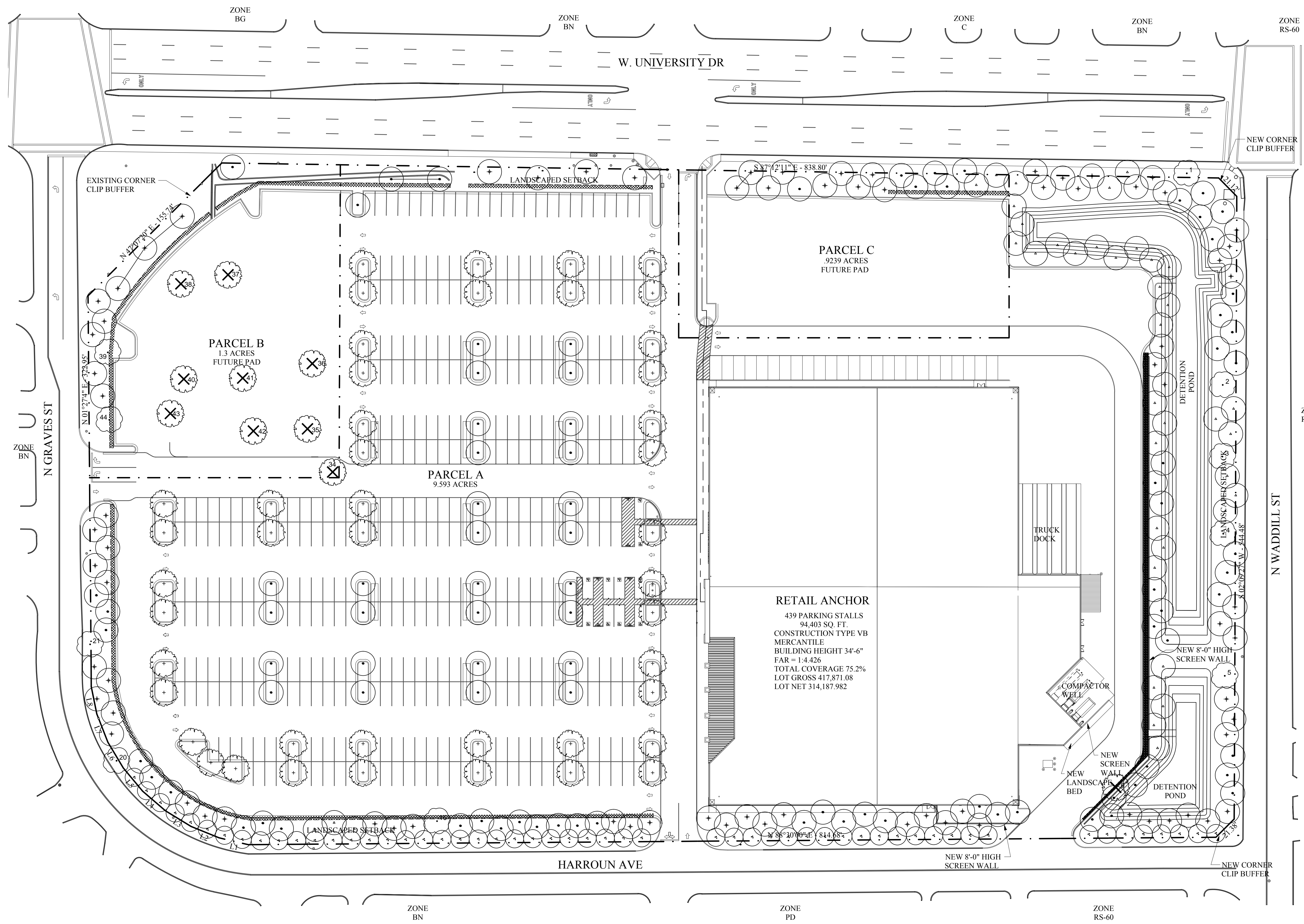
SITE PLAN 1" = 40'-0"
