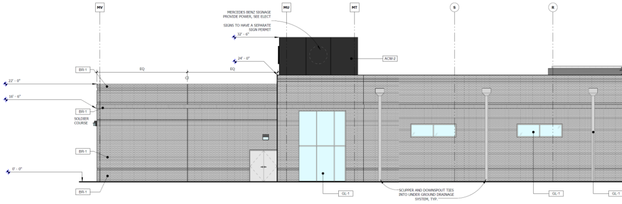
NORTH ELEVATION (REMAINDER OF THE BUILDING ELEVATION) BRAY CENTRAL DRIVE
