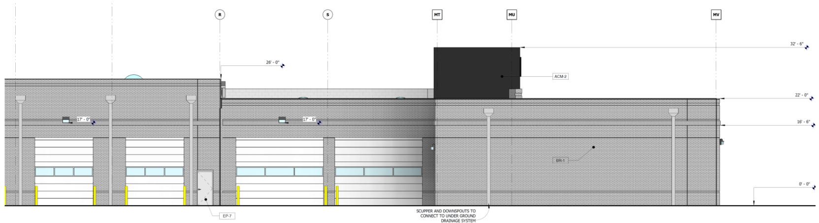
SOUTH ELEVATION (REMAINDER OF THE BUILDING)
