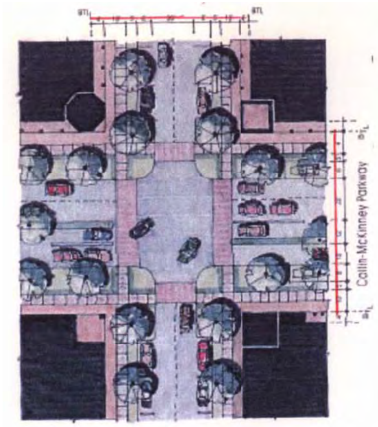
Pedestrian Bump-Out Diagram
