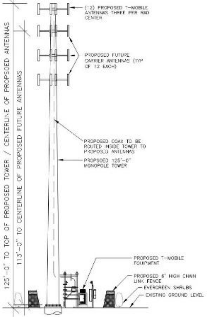
ENLARGED ZONING EXHIBIT
