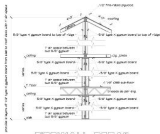
FIREWALL DETAIL SCALE NTS
