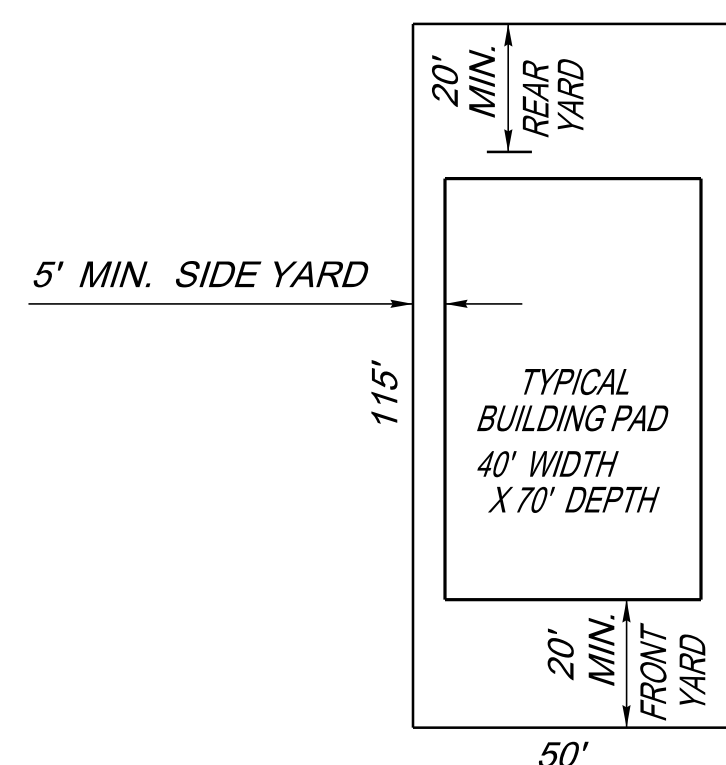
50 X 115 STANDARD LOT DIMENSIONS
