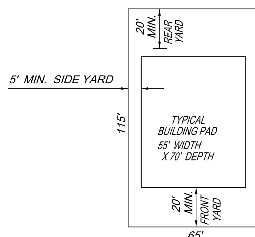
65 X 115 STANDARD LOT DIMENSIONS
