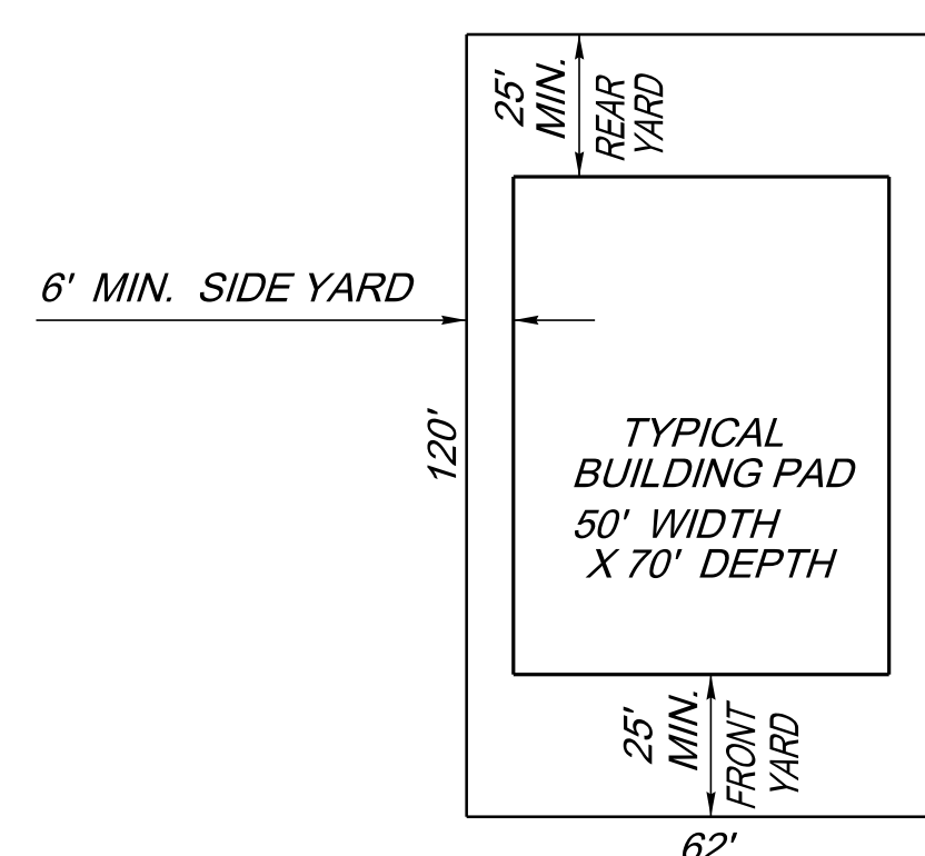
RS-72 STANDARD LOT DIMENSIONS
