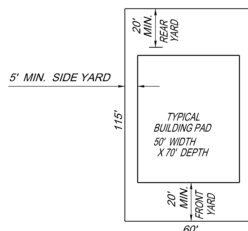
60 X 115 STANDARD LOT DIMENSIONS
