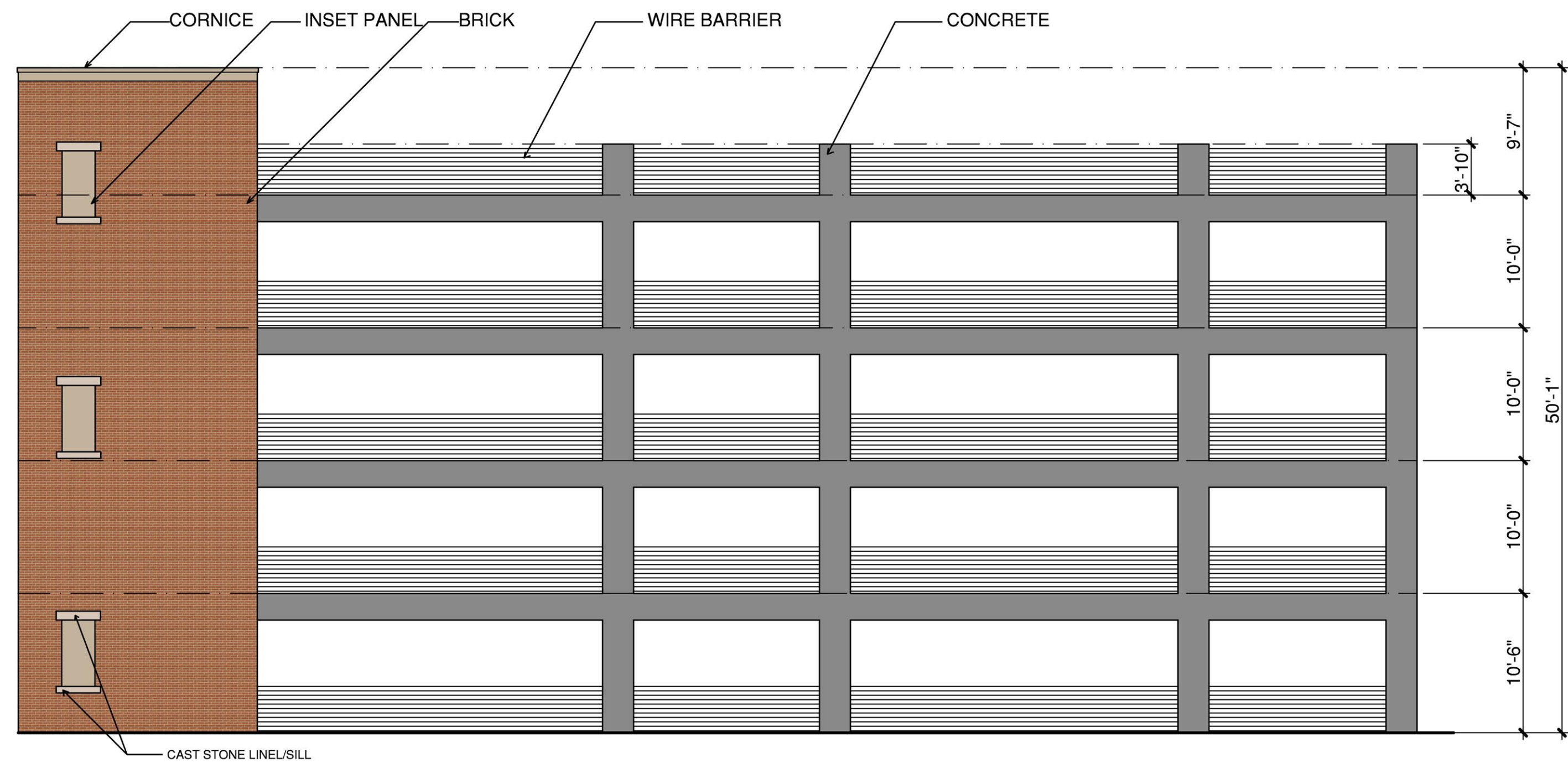
3 EAST GARAGE ELEVATION SCALE: 1/8" = 1'-0"
