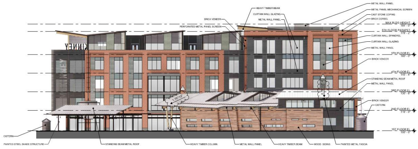
A1 EAST ELEVATION 1/16" = 1'-0"
