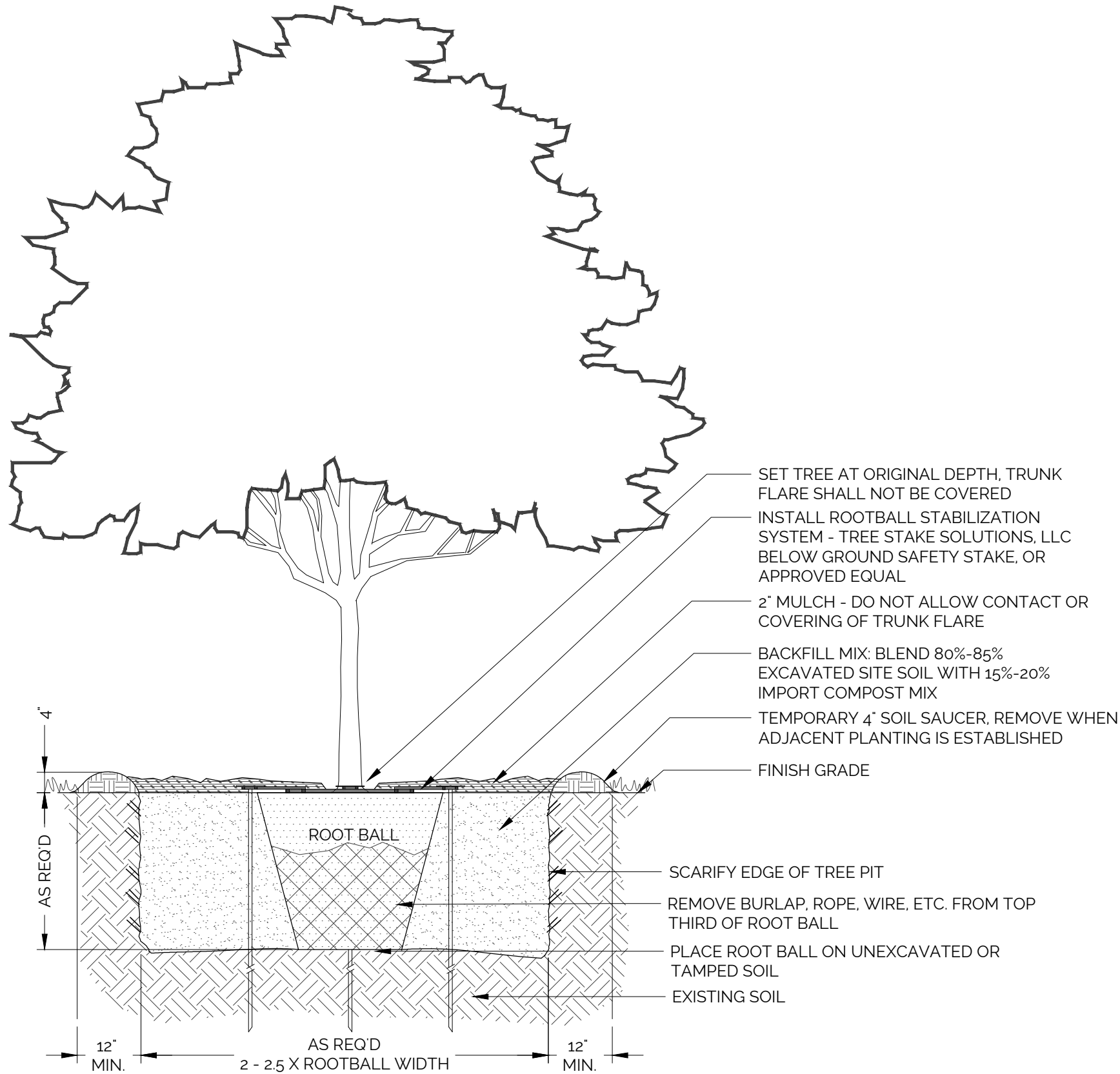
1 1/2"-1'-0" SHADE TREE PLANTING
