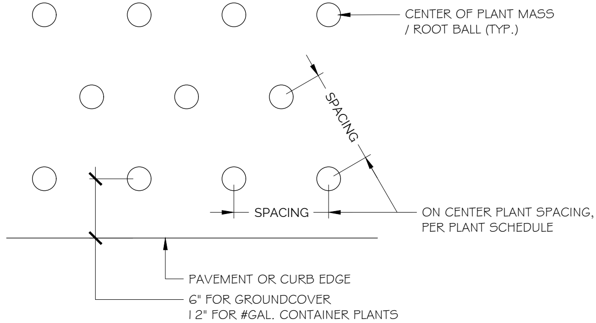
2 1/2"-1'-0" PLANT SPACING DIAGRAM
