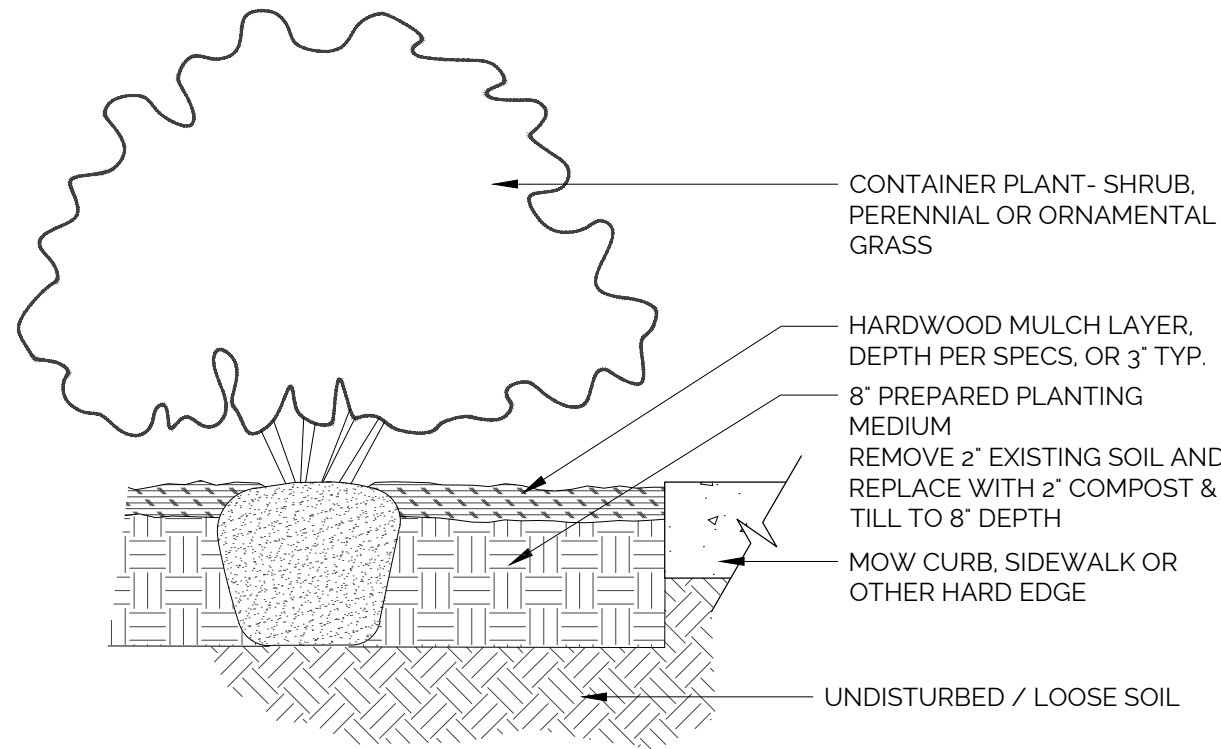
3 1'-1'-0" CONTAINER PLANTING
