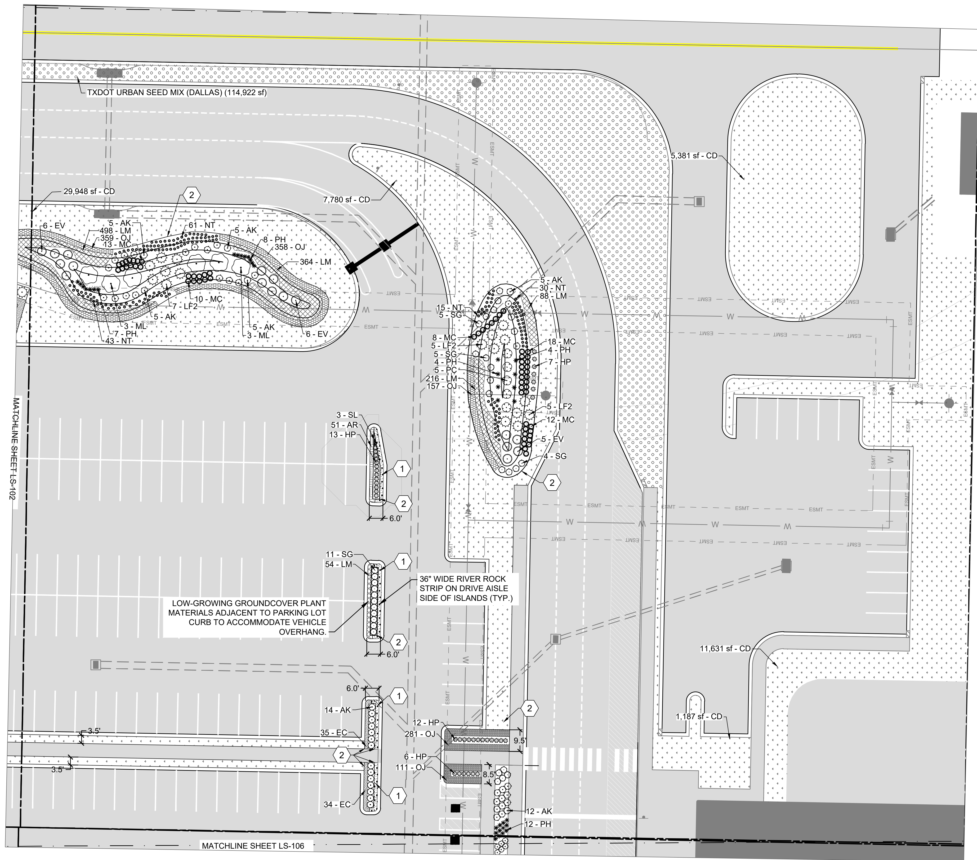
1 LANDSCAPE PLAN- SECTOR 3 SCALE: 1" = 20'
