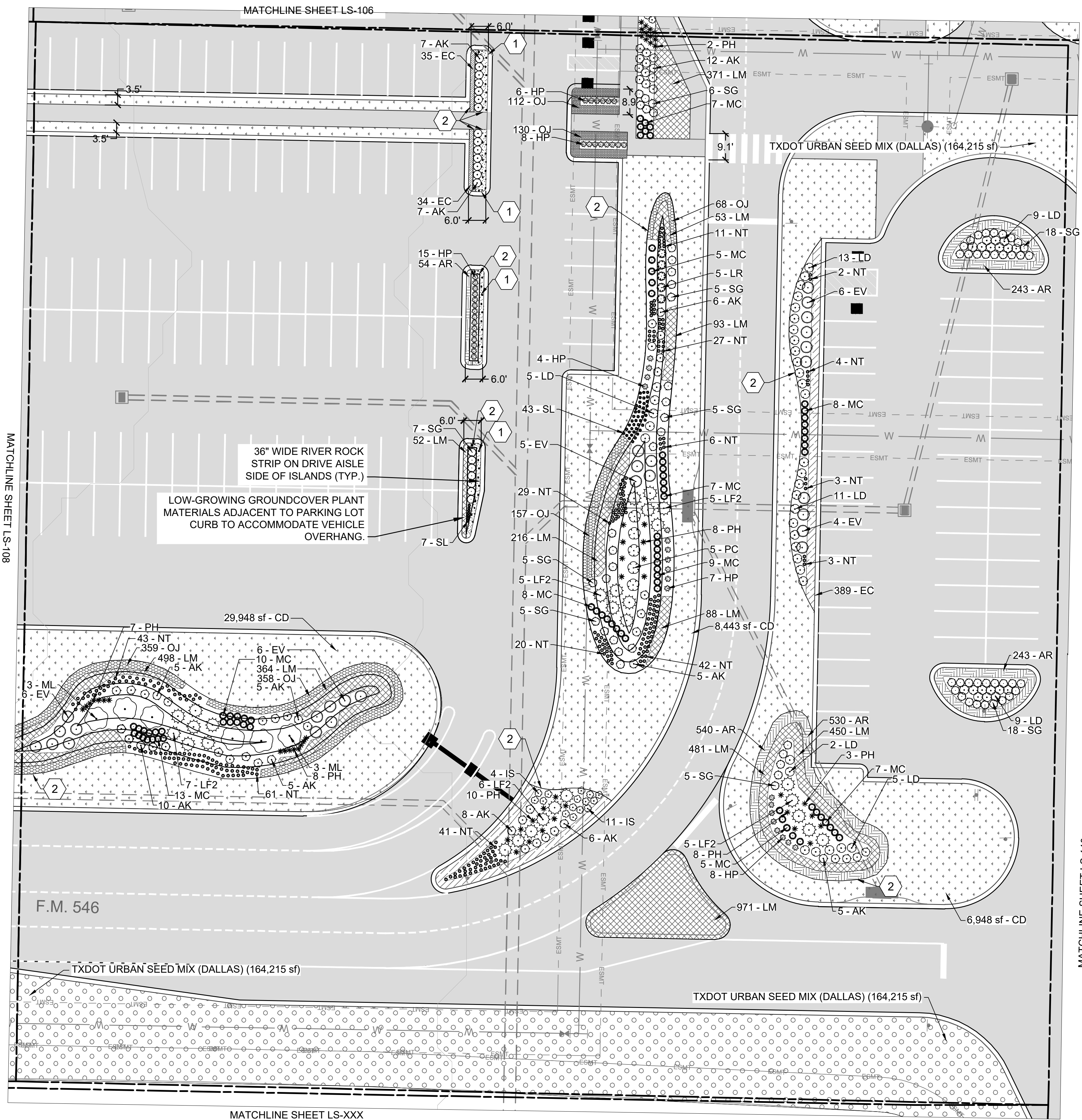
1 LANDSCAPE PLAN- SECTOR 9 SCALE: 1" = 20'
