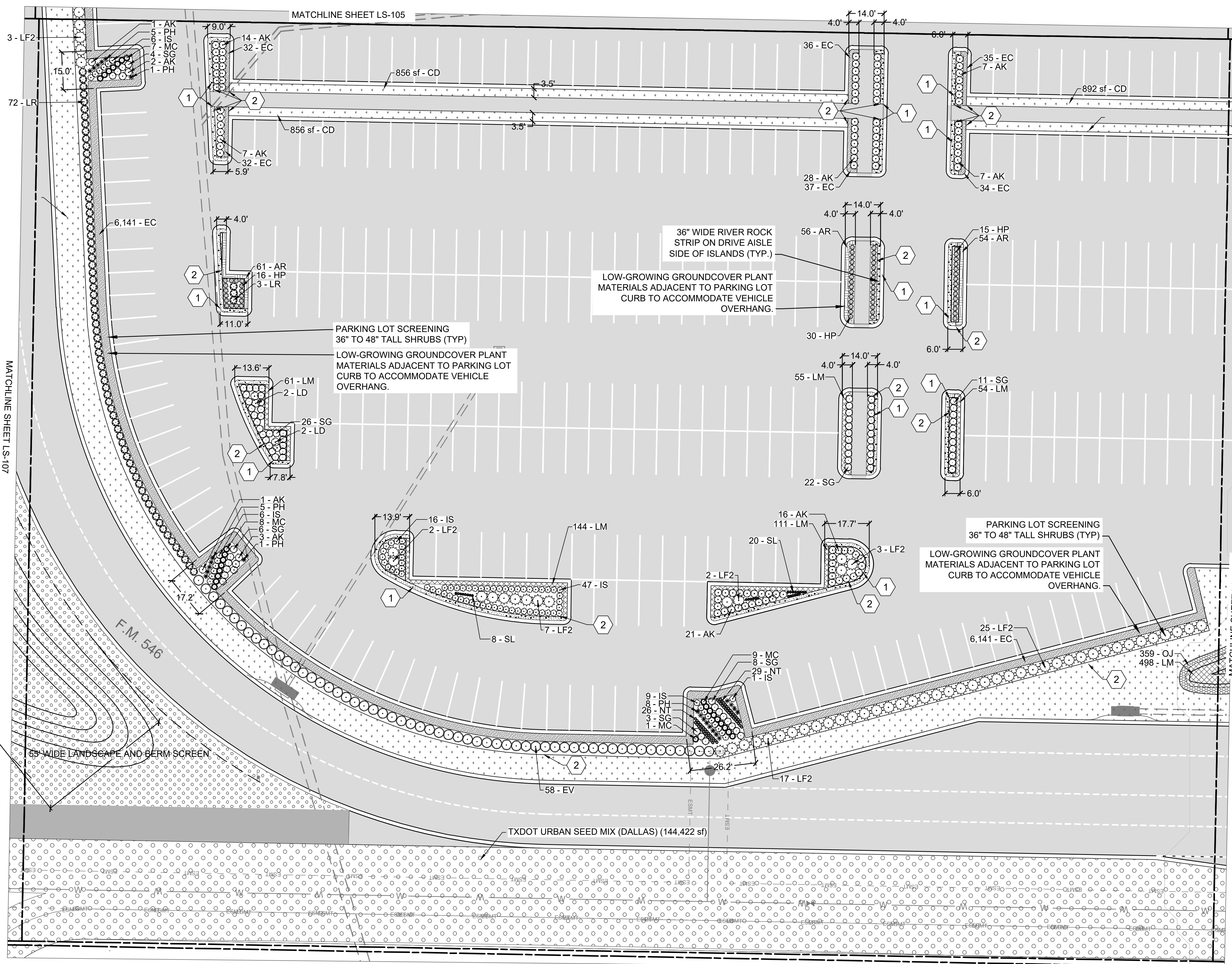
1 LANDSCAPE PLAN- SECTOR 8 SCALE: 1" = 20'
