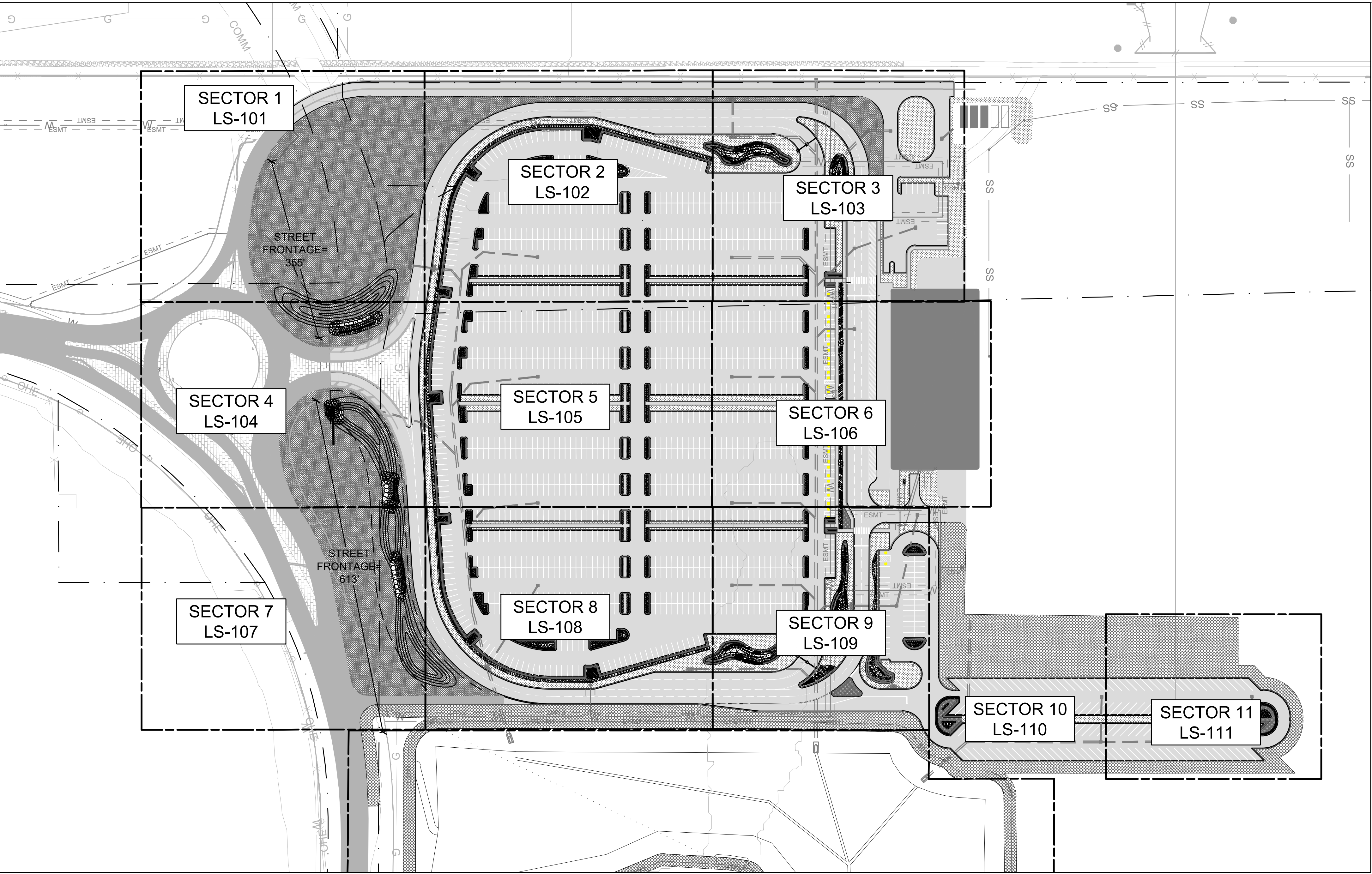
1 OVERALL LANDSCAPE PLAN SCALE: 1" = 100'
