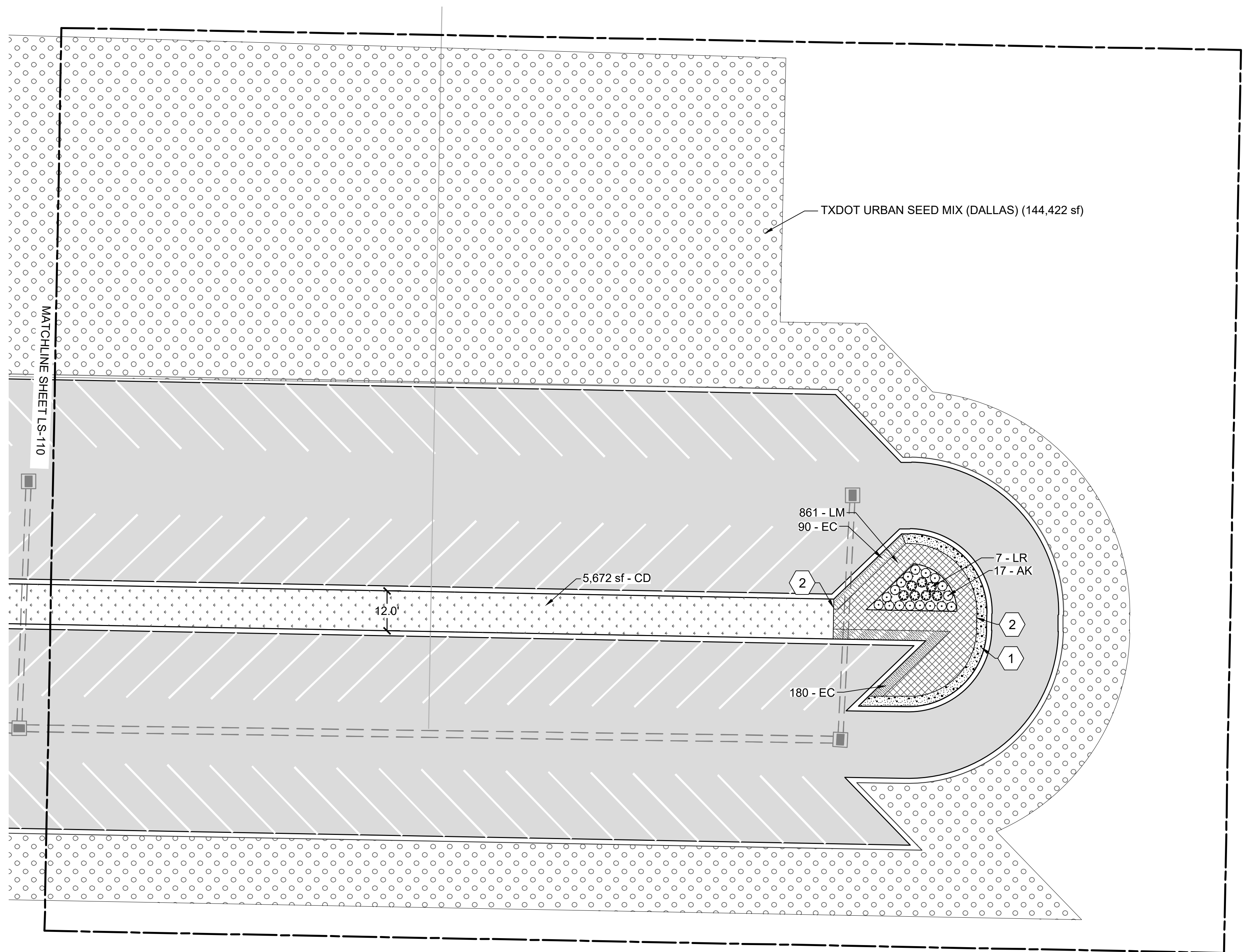
1 LANDSCAPE PLAN- SECTOR 12 SCALE: 1" = 20'
