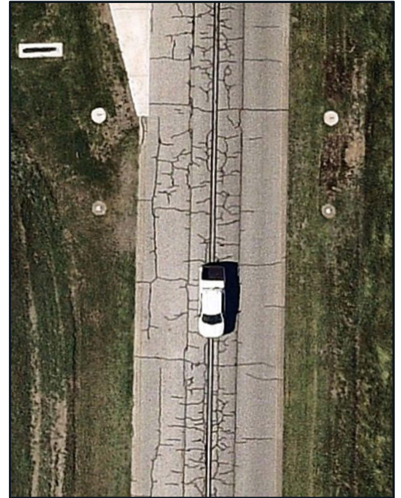
Segment of Taxiway A
