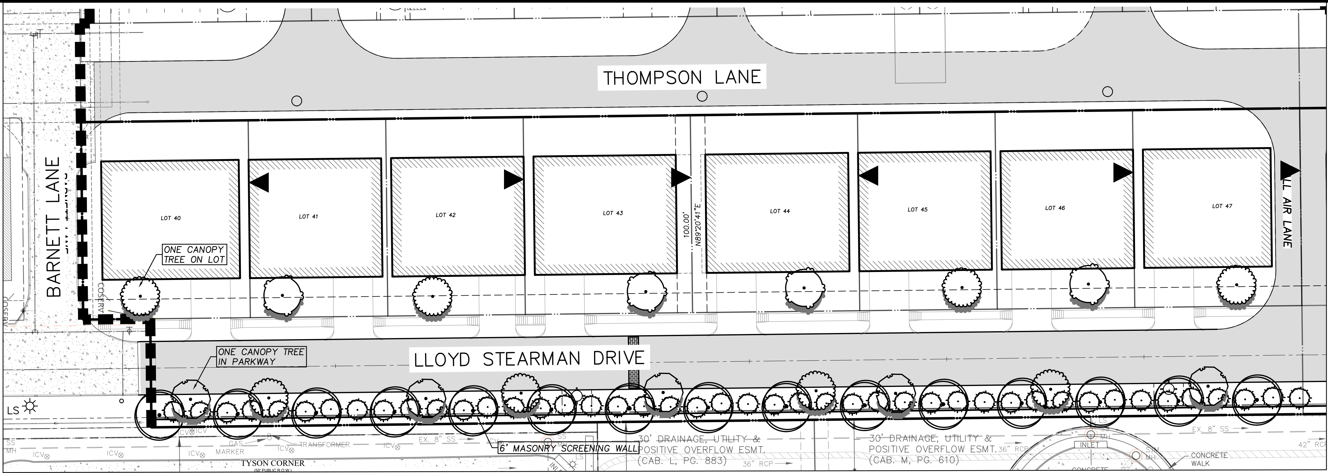
TYPICAL PLANTING ALONG SINGLE-FAMILY WITH HANGER AND EAST PROPERTY LINE
