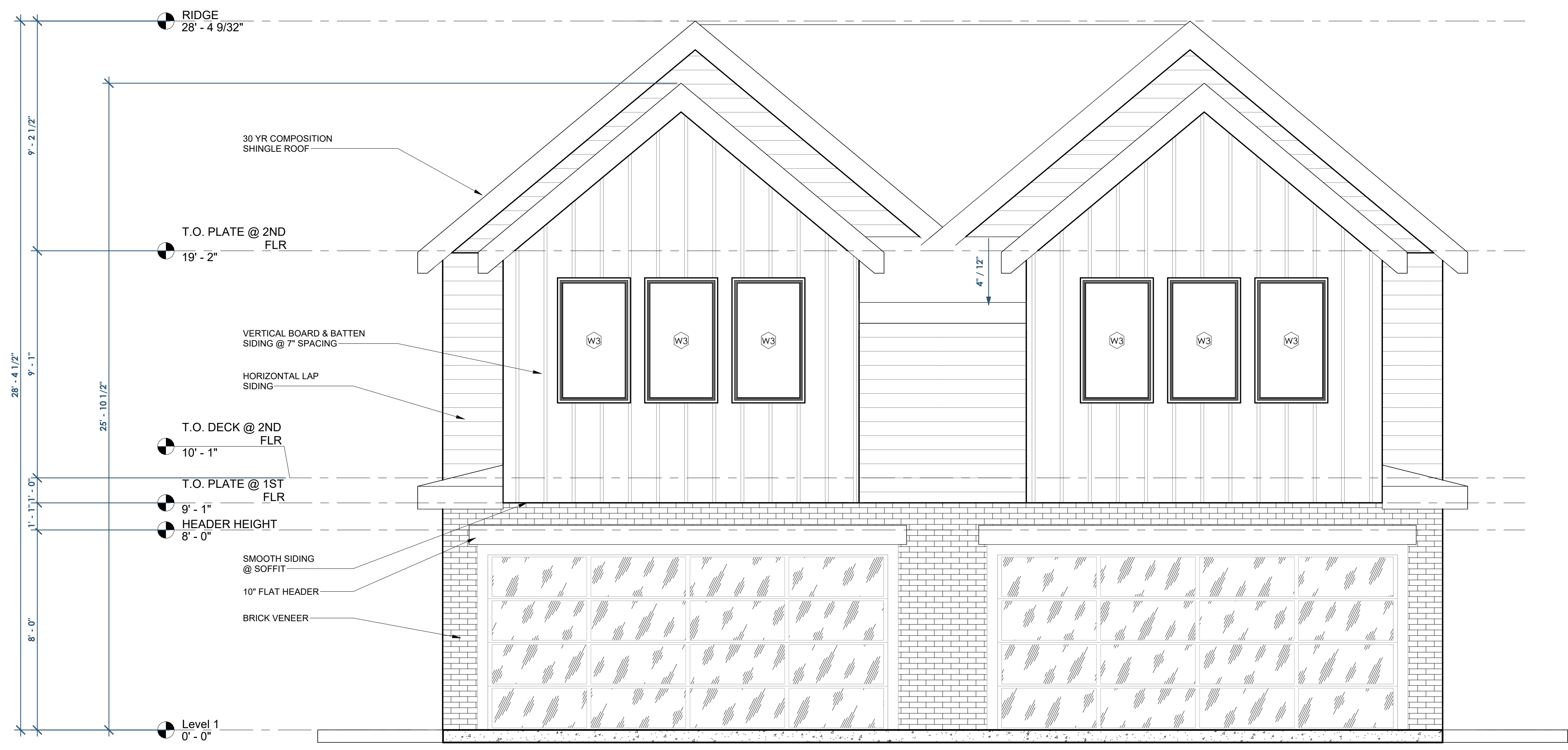
1 FRONT ELEVATION 3/8" = 1'-0"
