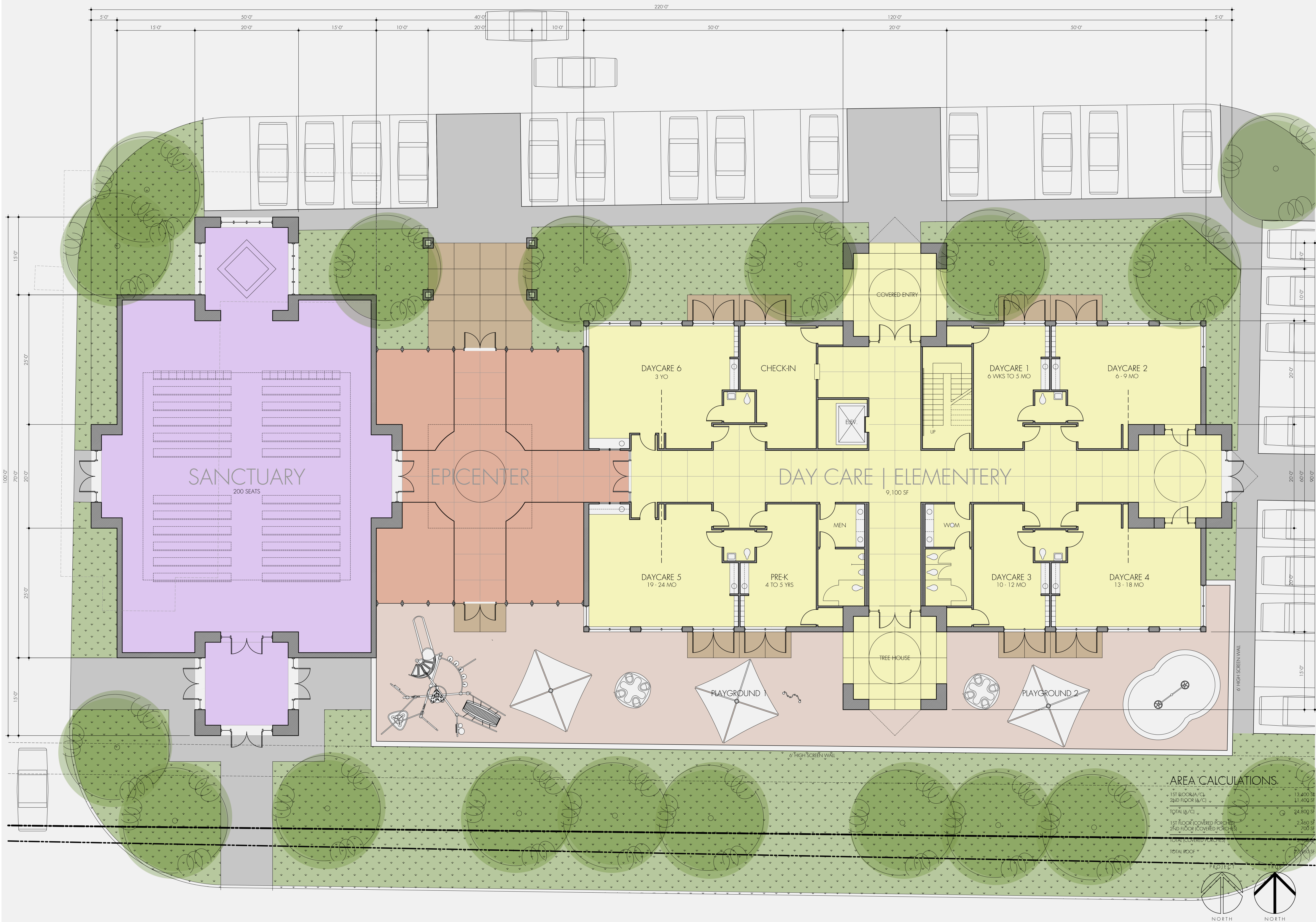
SCHEME 2 1ST FLOOR PLAN SCALE: 1/8" = 1'-0"
