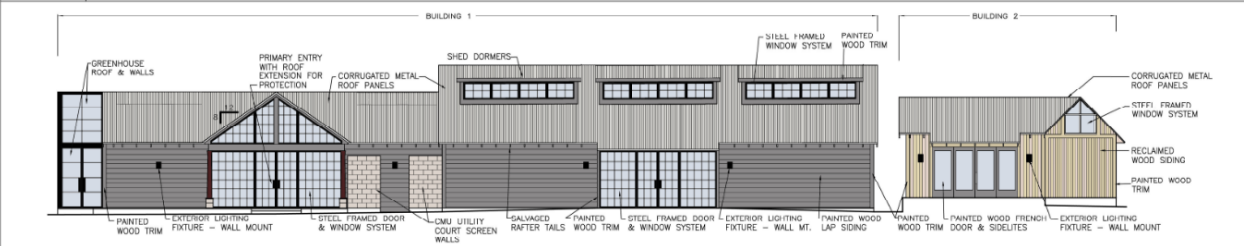
9 WEST FACADES 1/8"=1'-0" BLDGS. 1 & 2
