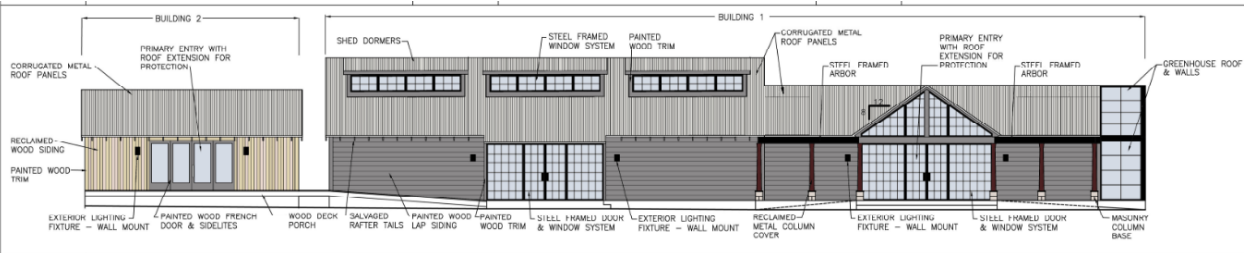
8 EAST FACADES 1/8"=1'-0" BLDGS. 1 & 2
