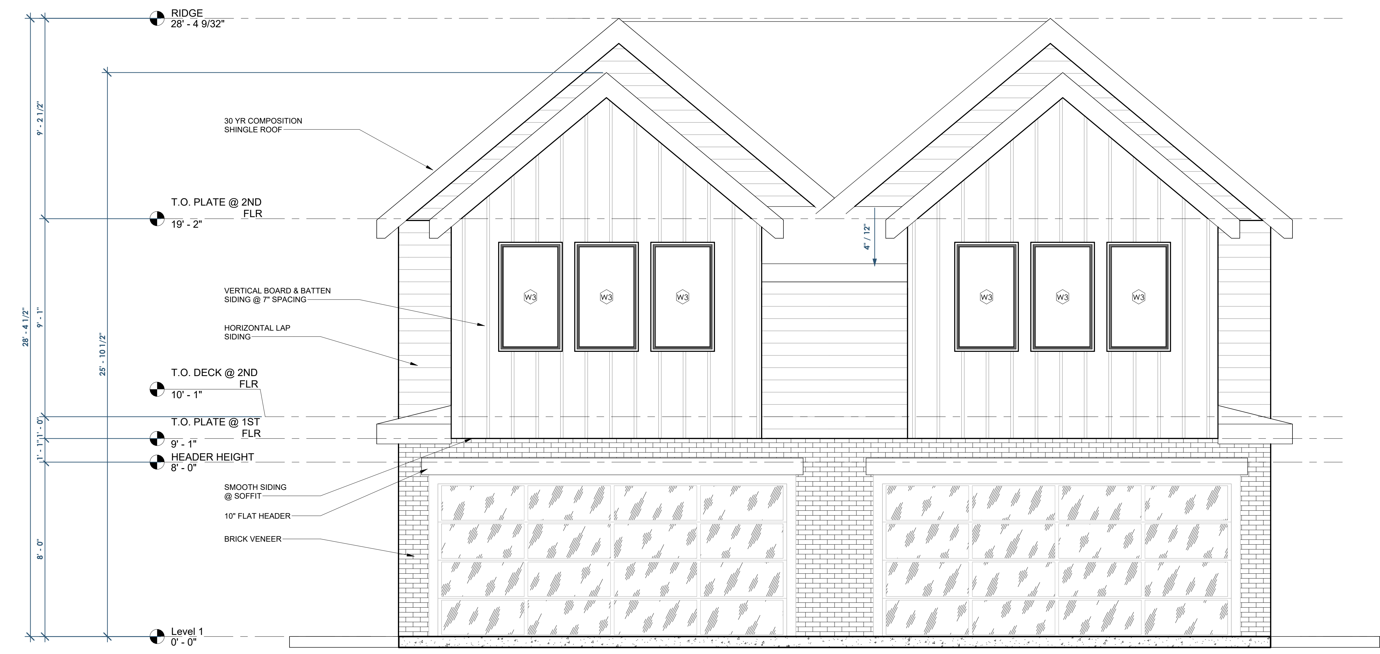
1 FRONT ELEVATION 3/8" = 1'-0"
