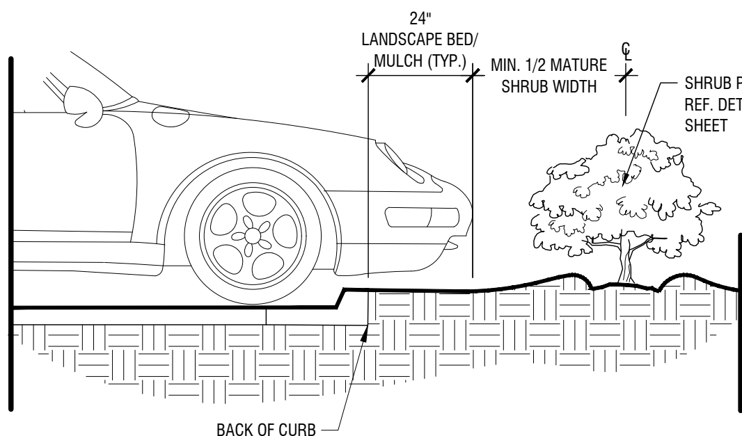
Shrub Planting at Curb
