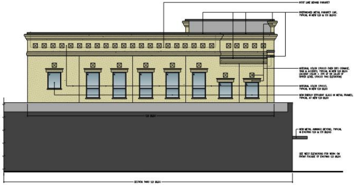
2 NORTH ELEVATION 1/4" = 1'-0"
