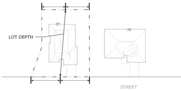
Figure 9-3: Lot Depth
