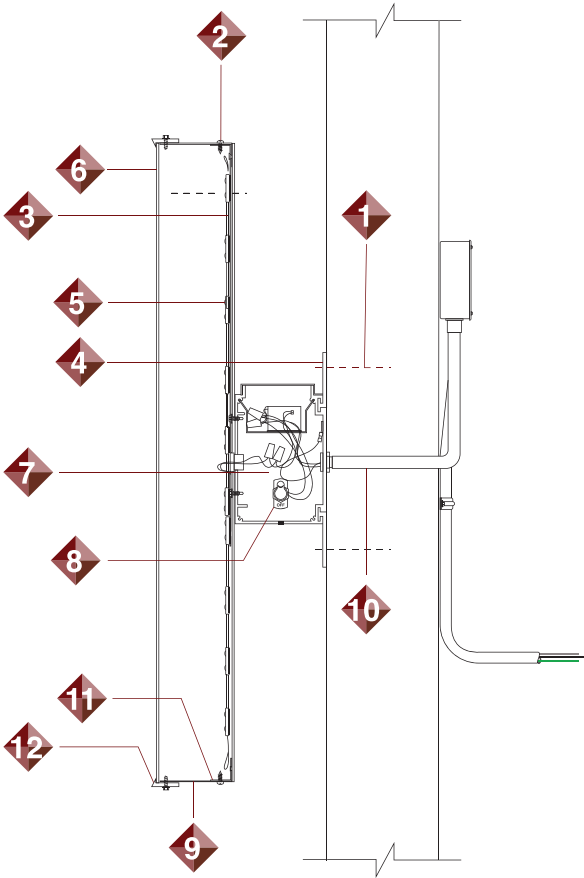
LED RACEWAY ASSEMBLY
