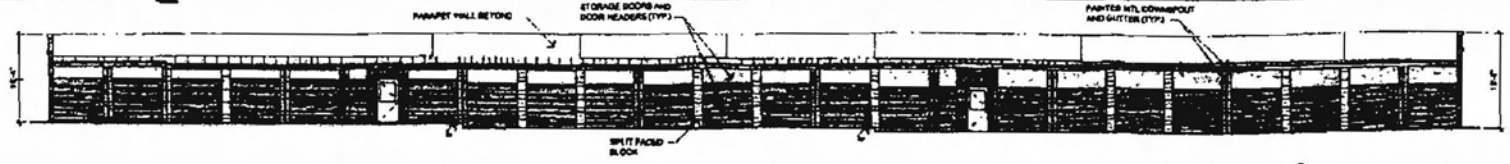
01 BUILDING C 302' x 42' NORTHWEST ELEVATION TOTAL MASONRY AREA PERCENTAGE: 100.0% OTHER: 0.0%
