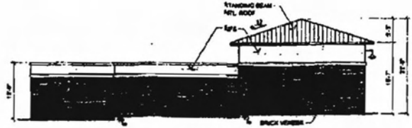
07 BUILDING B EAST ELEVATION
