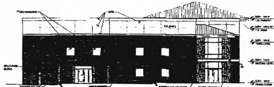
02 BUILDING A EAST ELEVATION TOTAL WINDOW AREA PERCENTAGE: 16.8% OTHER: 83.2%
