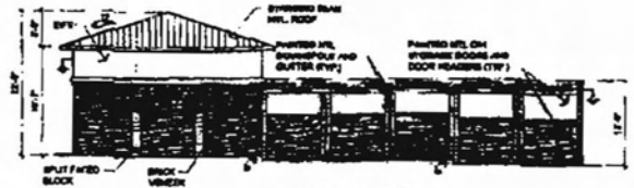
05 BUILDING B WEST ELEVATION TOTAL WINDOW AREA PERCENTAGE: 12.6% OTHER: 87.4%
