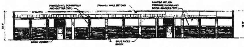
05 BUILDING D 302' x 42' NORTHEAST ELEVATION TOTAL MASONRY AREA PERCENTAGE: 98.0% OTHER: 2.0%
