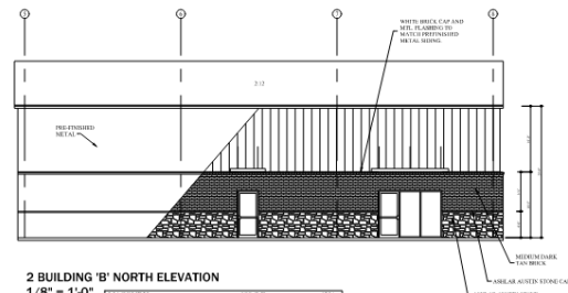
2 BUILDING 'B' NORTH ELEVATION 1/8" = 1'-0" MASONRY
