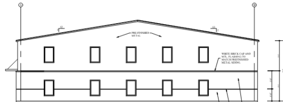
4 BUILDING 'B' WEST ELEVATION 1/8" = 1'-0" MASONRY
